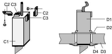
Figure 4: Mounting the receiver
