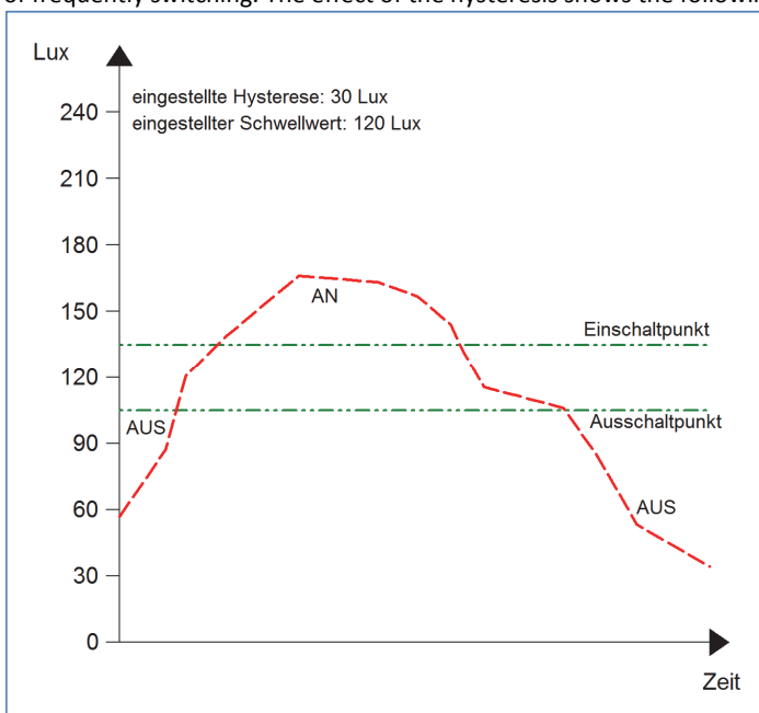
Figure 8: Hysteresis brightness threshold
