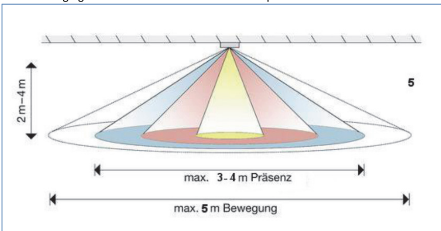
Figure 2: Detection area SCN-P360x4.01 Figure 3: Detection area SCN-P360x3.01
