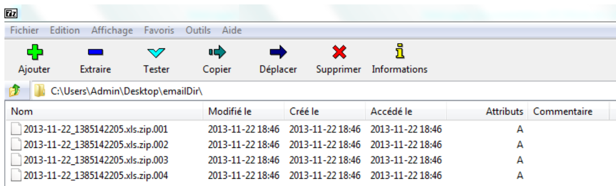
Figure 18: 7zip
