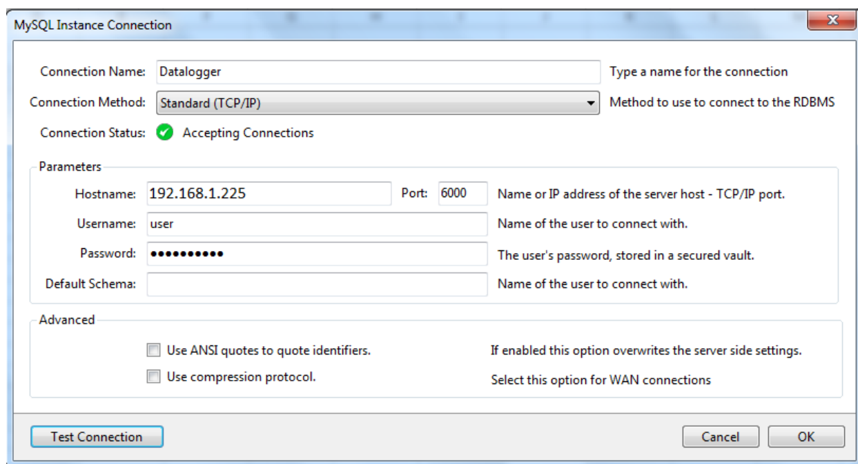
Figure 31: Add database connection
