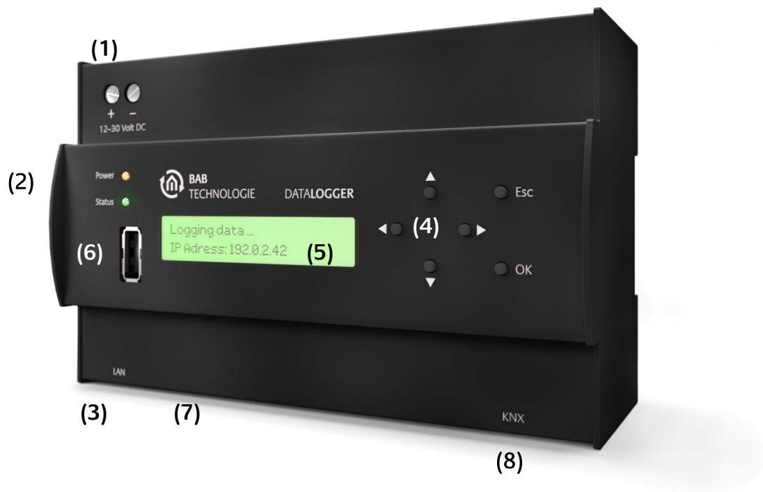
Figure 1: Device Overview
