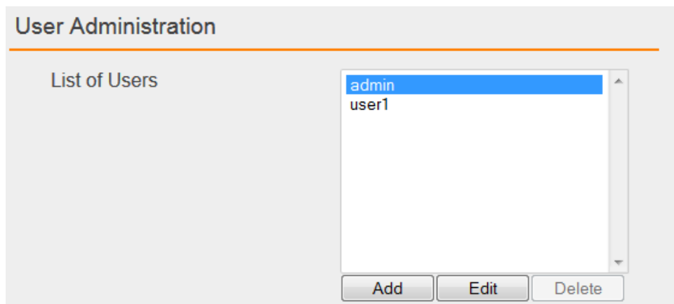
Figure 7: User Administration
