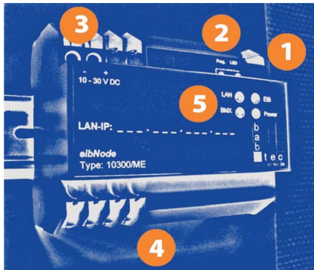
figure 1: eibNode Data links/Ports
