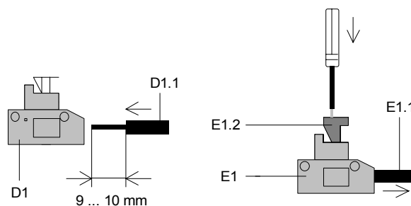
Figure 5: Connecting and disconnecting the cable
