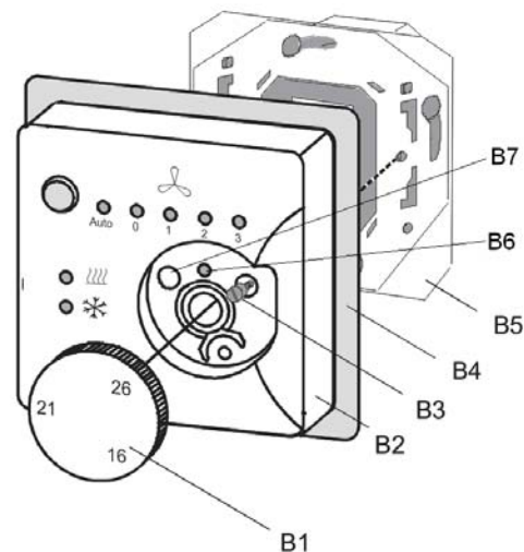
Figure 3: Mounting the FCU Operator Panel Hotel
