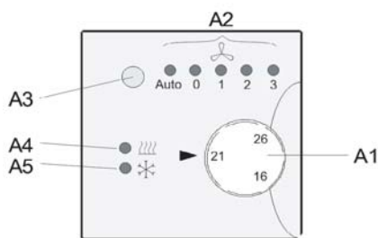
Figure 2: Position of the operating and display elements
