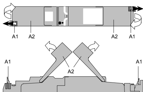
Figure 2: Opening and closing the cover lids
