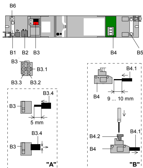
Figure 3: Connections
