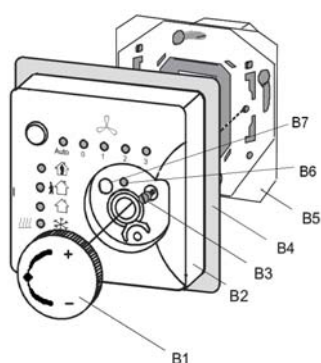
Diagram 3: Mounting the FCU Operator Panel Office
