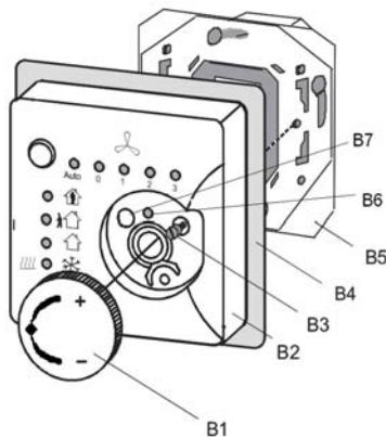
Diagram 1: Mounting the Fan-Coil Unit Operator Panel
