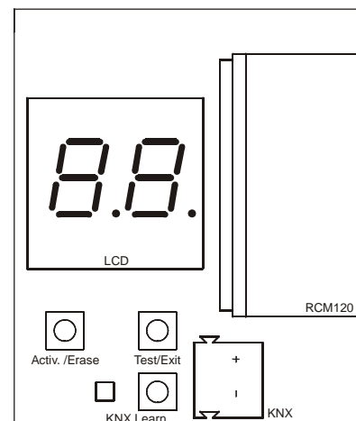
Fig. 5: Device with top open
