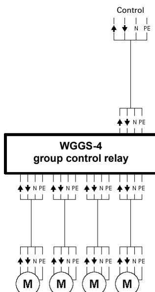
WGGS-4 group control relay
